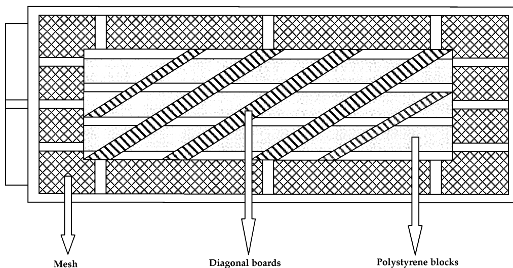
Underside view
